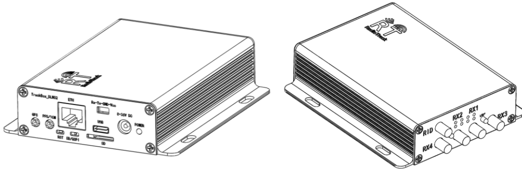
Figure 1: Module Appearance
